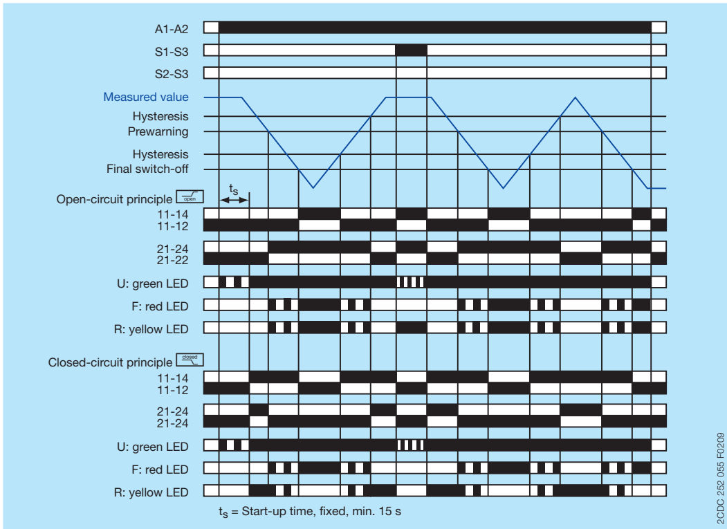
Insulation resistance monitoring w/o fault storage , auto reset, 2 x 1 c/o
