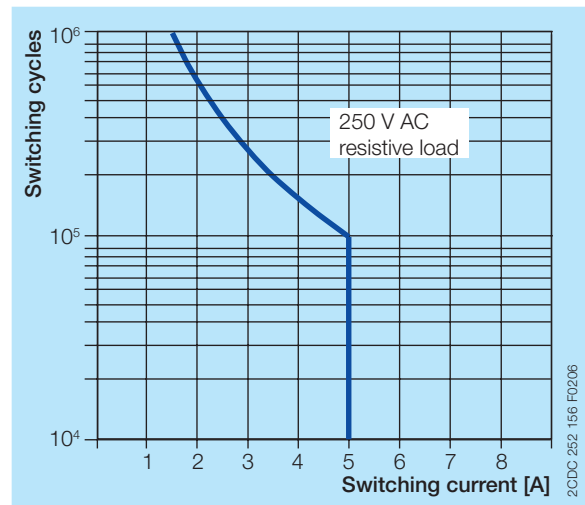
Contact lifetime
