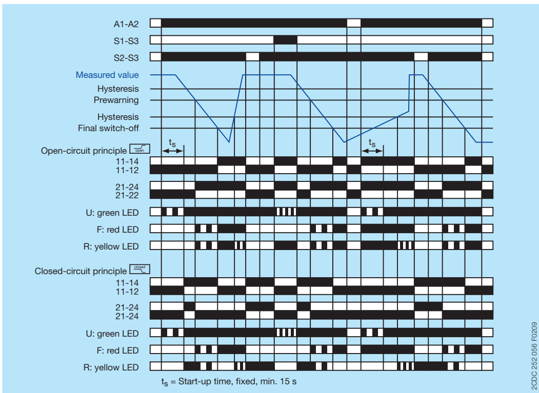
Insulation resistance monitoring with fault storage , manual reset, 2 x 1 c/o
